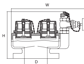
2 Way Breeching
