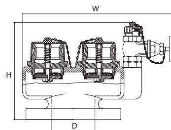
4 Way Breeching
